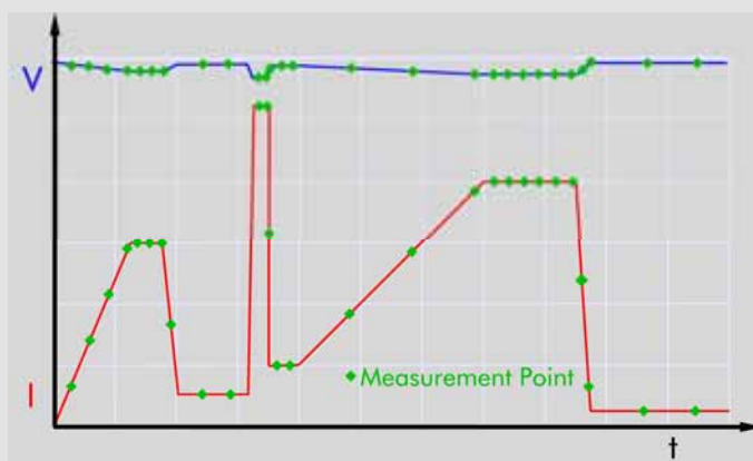
Data acquisition with variable reading rate synchronized with the programmed waveform. Simultaneous reading of voltage and current.
